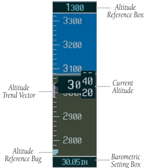
Figure 3.4.6 Altimeter
