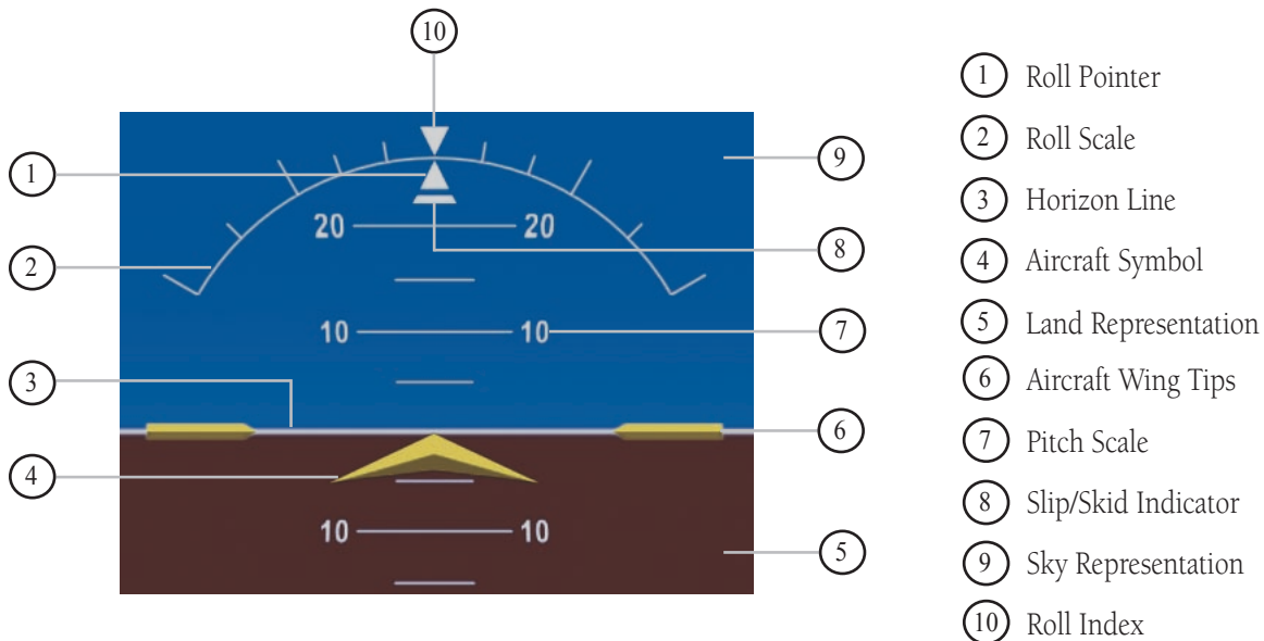
Figure 3.4.3 Attitude Indicator
